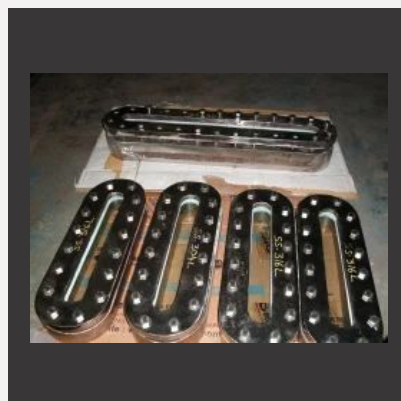
Weld Pad Level Gauge
